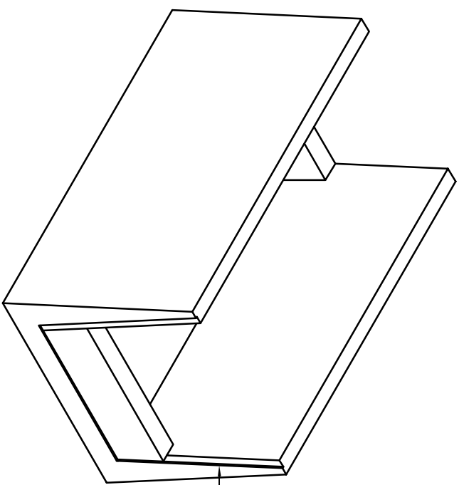
ISOMETRIC VIEW - SLURRY CHAMBER: (ROOF SLAB OMITTED FOR CLARITY)
