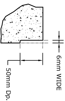
SECTION - TYPICAL GROOVE (ONE END ONLY) SCALE: 1:5
