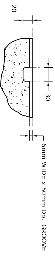
DETAIL A - PLAN VIEW AT VERTICAL GROOVE SCALE: 1:5
