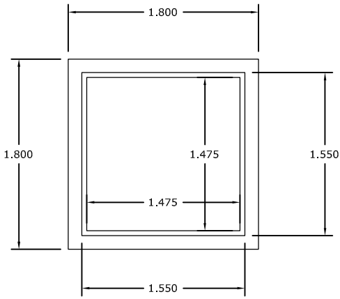
RIM PLAN
