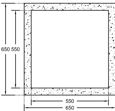
BASE PLAN VIEW SCALE: 1:15
