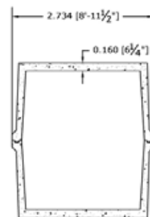
SHORT SECTION
